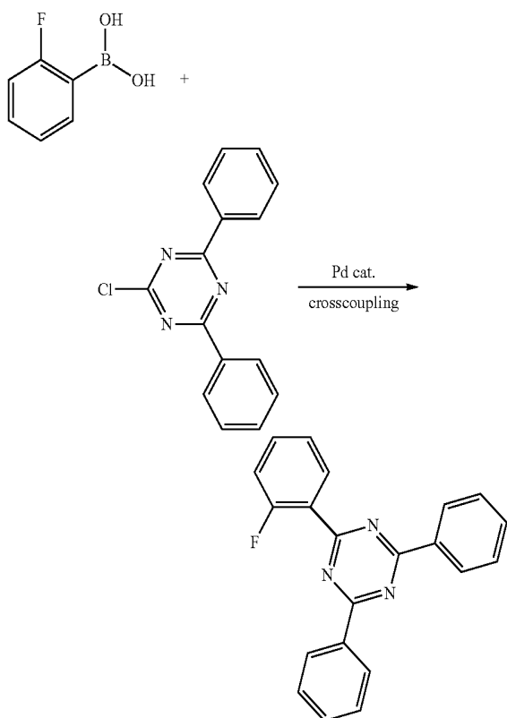
[Scheme 5]
