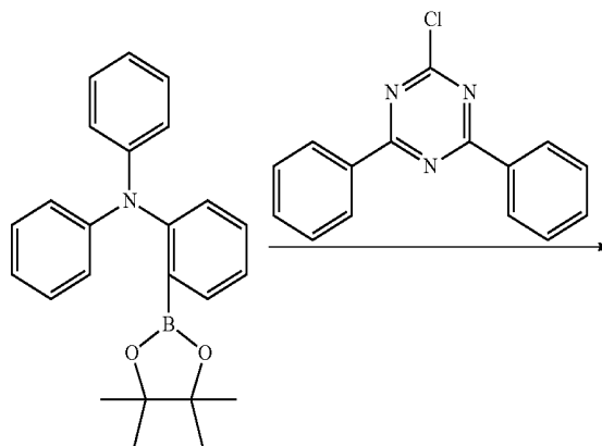
[Scheme 2-3]
