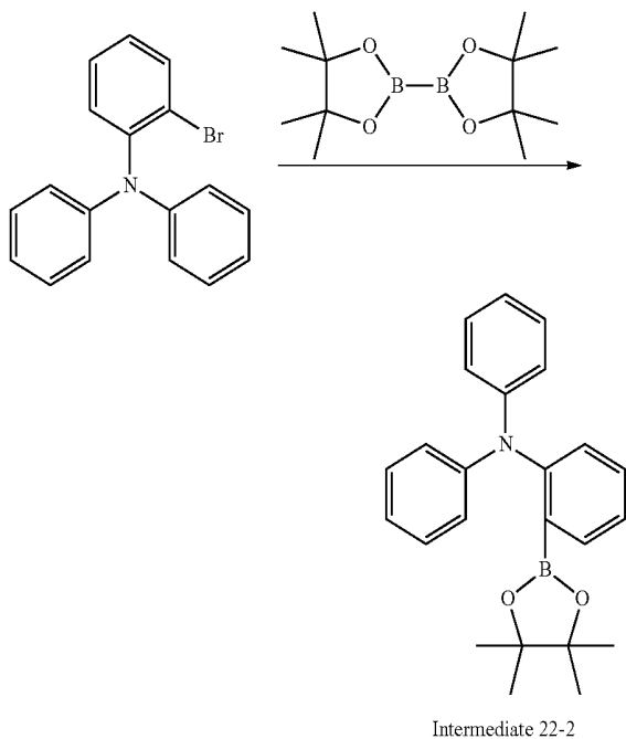
[Scheme 2-2]
