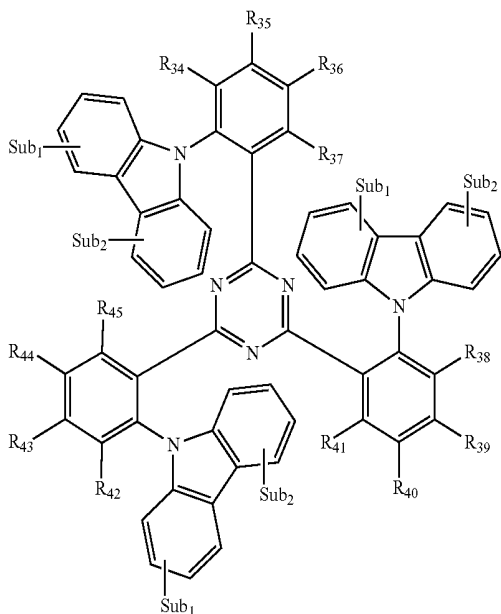
[Chemical Formula 12]
