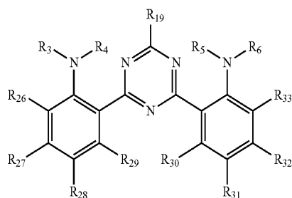
[Chemical Formula 3]
