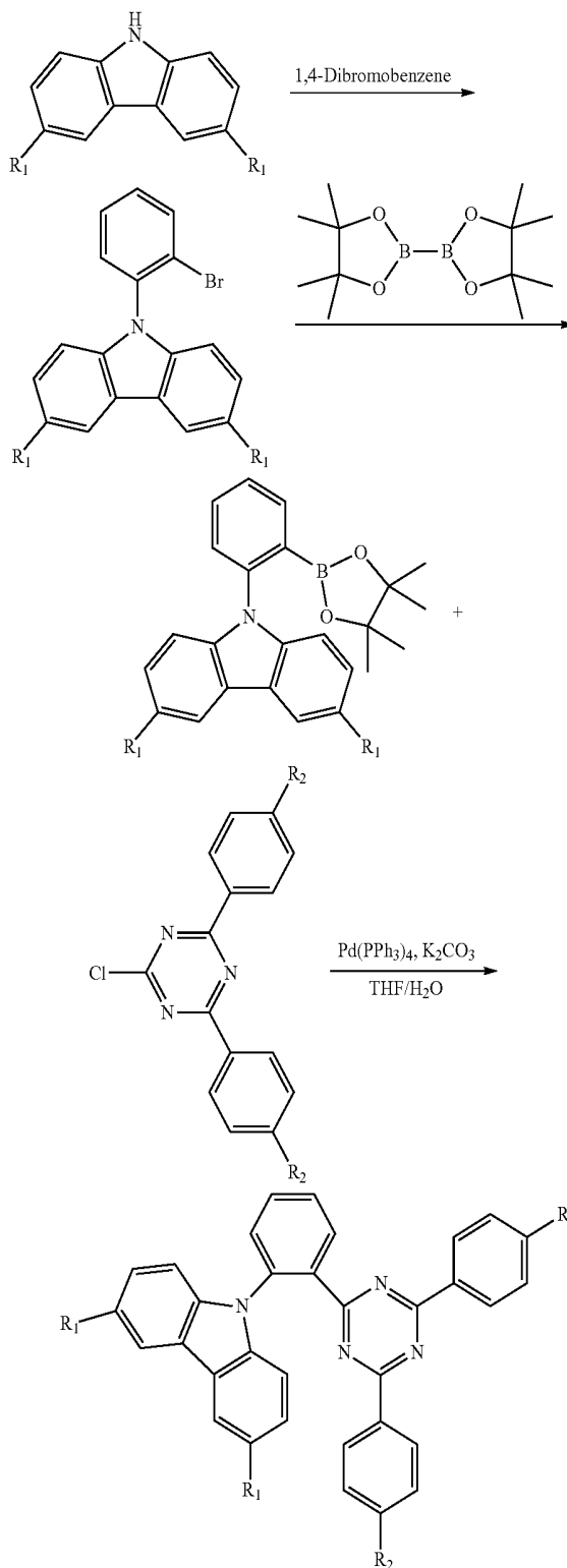
Scheme 1
